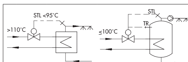
Fig. 1: DHW heating according to DIN 4753
