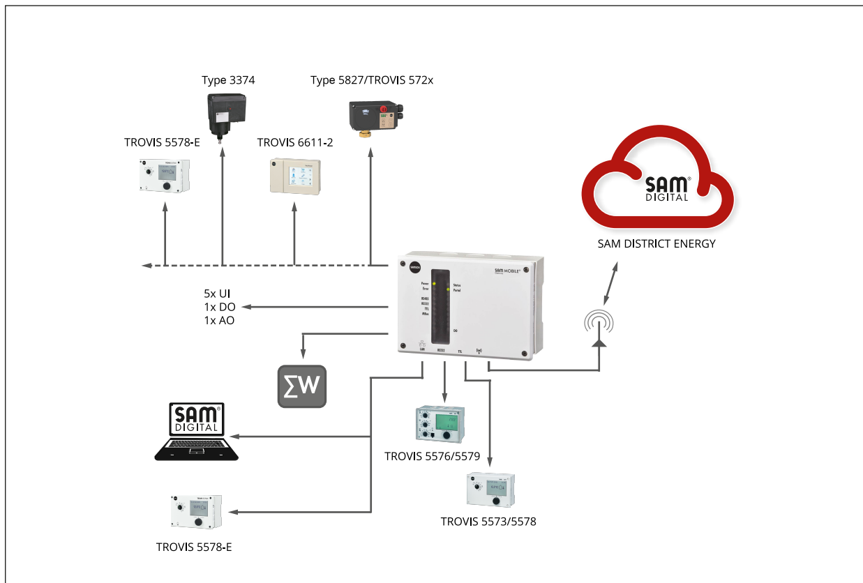
Fig. 1: Application using the SAM MOBILE+ Gateway
