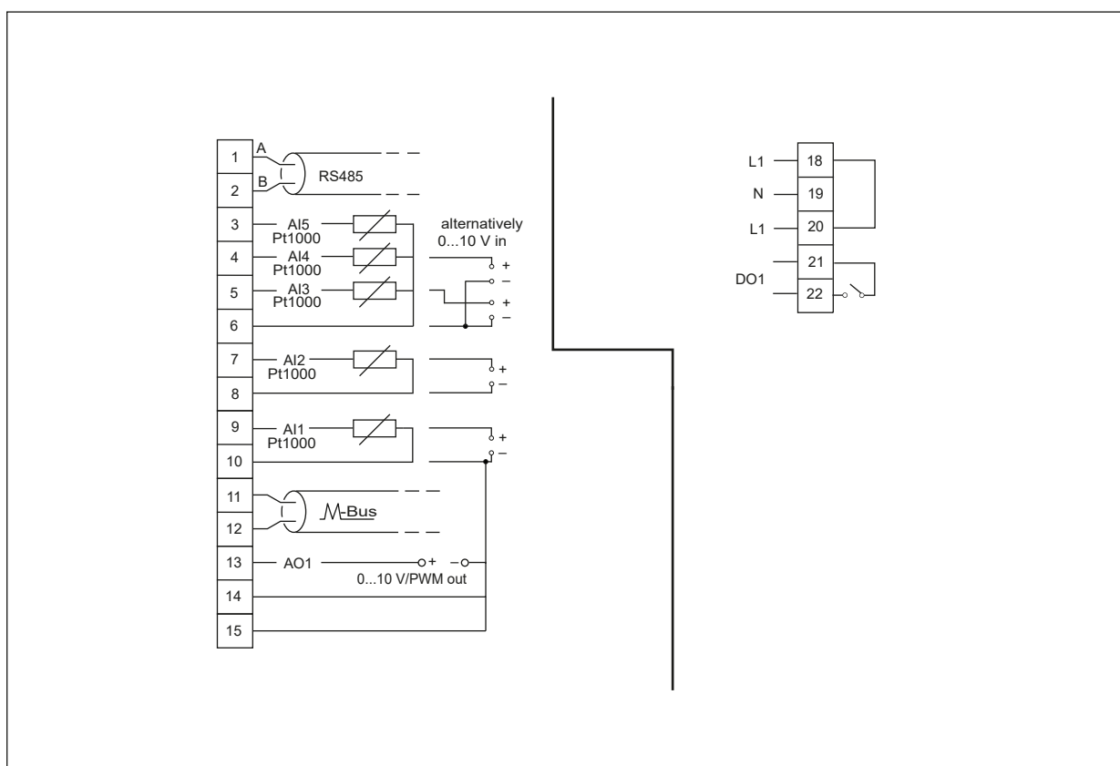
Fig. 5: Electrical connection · Type 5656
