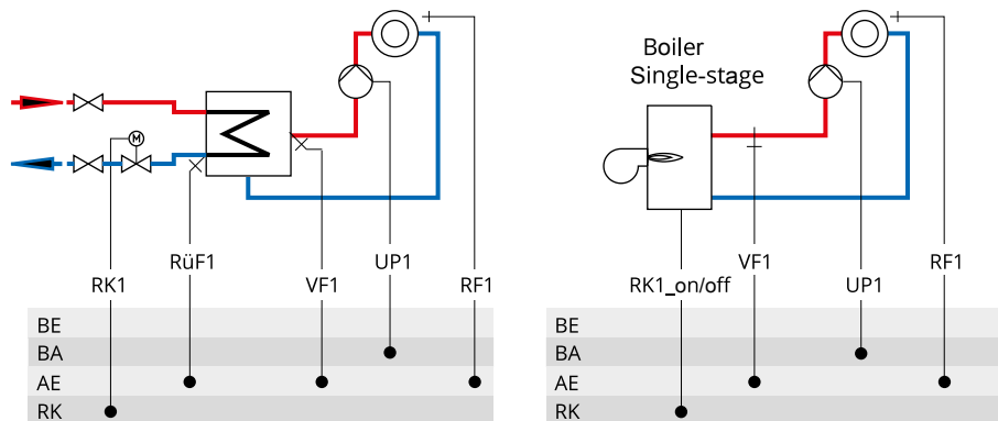
Fig. 14: Configuration of a boiler system
